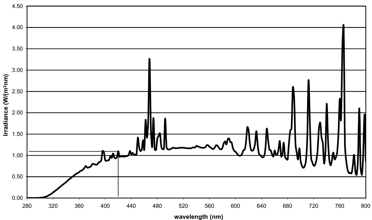
Fig. A1—Filtered Xenon Lamp Spectral Power Distribution Controlled at 1.1 W/(m 2 nm) at 420 nm
